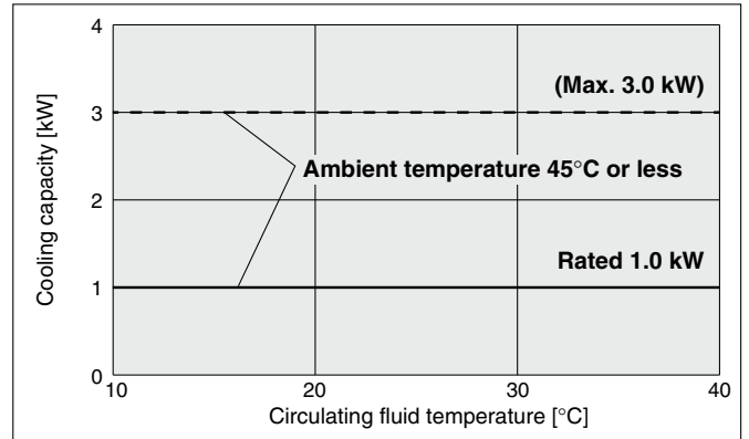
HRL200-W□-40-T2 (CH1)*1
