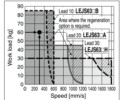
<Speed-Work load graph> (LEJS63)
