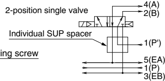
Circuit diagram (Mounting example of a 2-position single valve)
