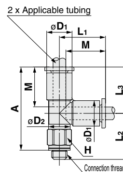
Release button dimensions
