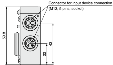
EX250-IE1
