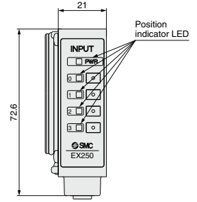
EX250-IE2
