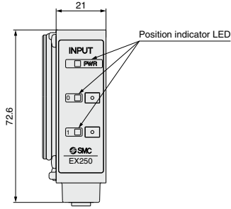
EX250-IE1
