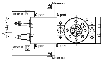
Figure 1 3-position pressure center solenoid valve: 1 pc.
