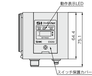
EX250-SDN1 (DeviceNet®)
