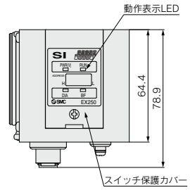
EX250-SPR1 (PROFIBUS DP)
